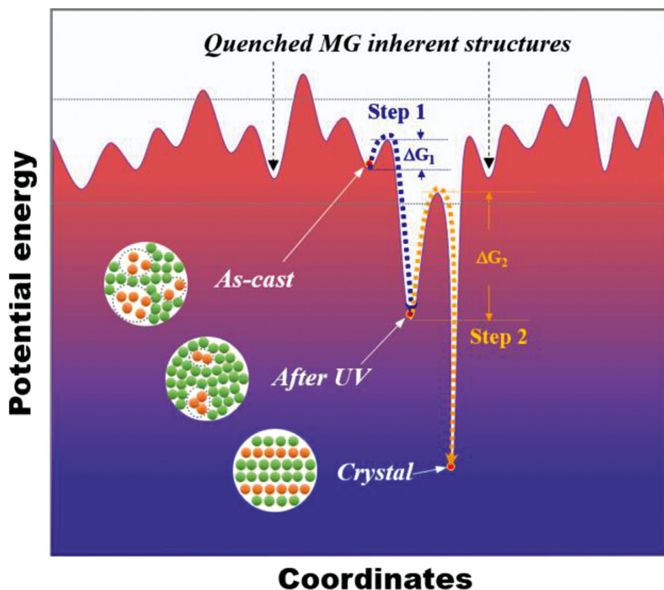
Fig. 5. Schematic diagram of the structure evolution and stabilization processes under UV in the potential energy landscape. The as cast MG quenched in a local basin with relatively higher energy. After UV at suitable energy, it can cross over an energy barrier \Delta G_1 and stabilize into a denser atomic packing state. With an even larger UV energy, the MG will climb over a higher energy barrier \Delta G_2 into stable crystalline state. Insets depict the atomic structure evolution after UV processing and crystallization. The orange atoms represent anelastic region that loosely pack and embed in solid glassy matrix (green atoms). (For interpretation of the references to color in this figure legend, the reader is referred to the web version of this article.)
