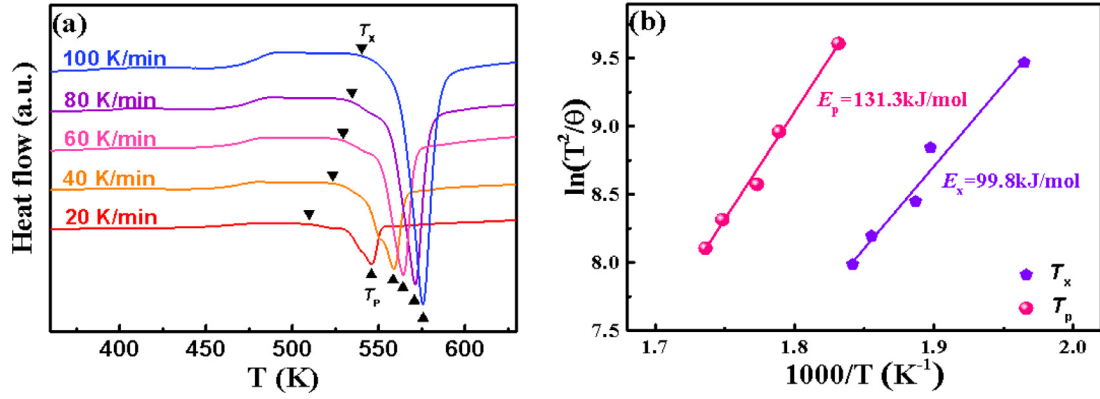
Fig. 4. The crystallization behavior of as-cast sample at different heating rates. (a) The changes in glass transition temperature T_g , crystallization onset temperature T_x and crystallization peak temperature T_p . (b) The estimation of the activation energy of the two exothermic events by using Kissinger equation.
