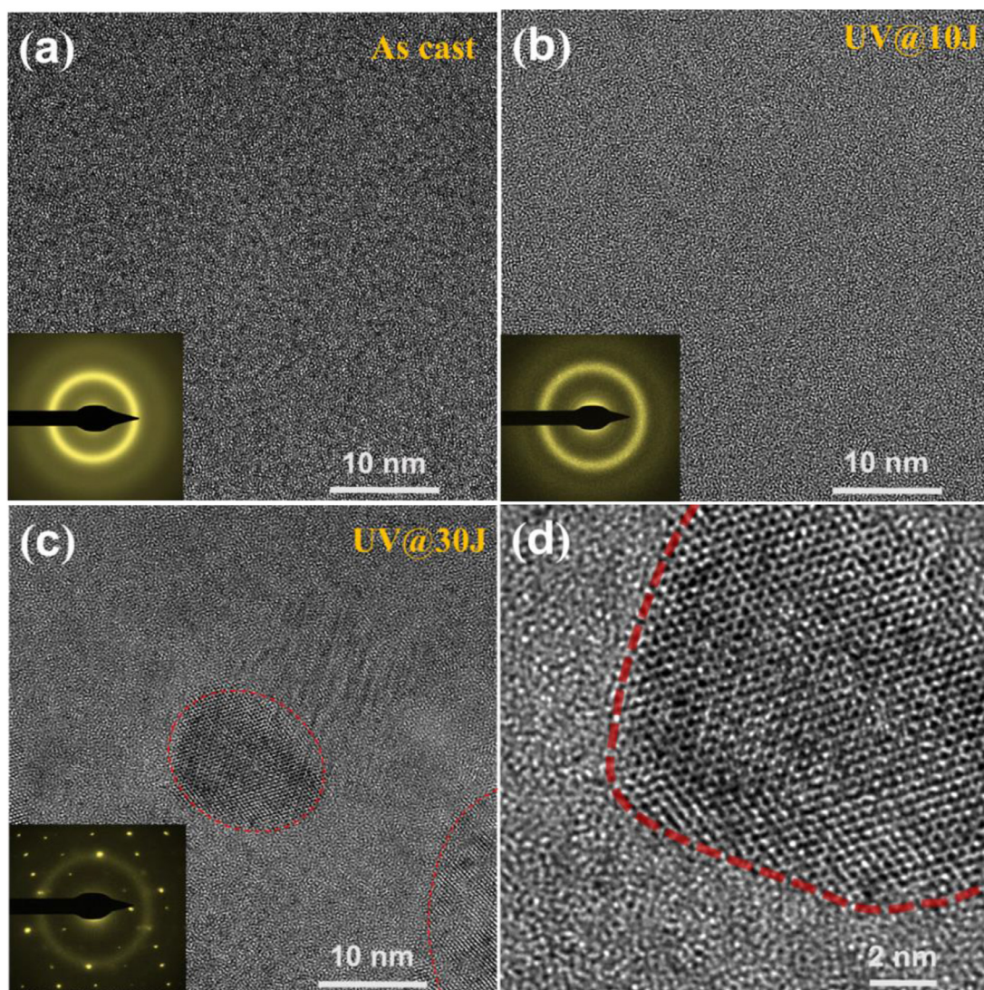
Fig. 2. Structure characterization of the as cast and UV processed samples. HRTEM of (a) as cast MG, (b) MG after UV treatment with energy of 10 J and (c) 30 J. Insets: SAED patterns taken from a large selected area. The red dotted line in (c) exhibits the nanocrystal embedded in the MG matrix. (d) An enlarged image of the atomic structure of the 30 J UV processed sample. The red dotted thick line shows a clear boundary between nanocrystal and amorphous matrix.
