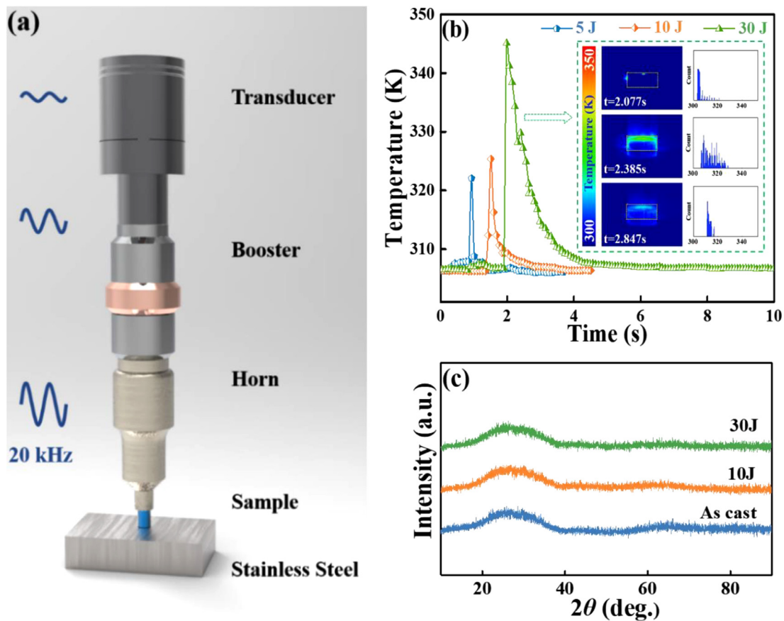
Fig. 1. Schematic diagram of ultrasonic treatment process and the variation of temperature and structure of the samples. (a) Ultrasonic vibration process sketch: ultrasonic vibration with 20 kHz is transmitted to the horn, and the horn exerts pressure and vibration on the sample. (b) The temperature variation of the samples obtains by high precision infrared thermometer during the ultrasonic process with different energy. The inset shows the temperature profile at different moments during UV at 30J. (c) XRD patterns for as cast sample and processed samples, which show no observed crystallization occurred.
