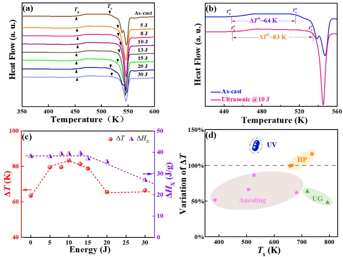
Fig. 3. The thermodynamic evolution behavior of La-based MG at various input energy. (a) The contrast DSC traces of as cast sample and UV samples with various input energies. For each alloy, the arrow pointing upwards indicates the glass transition temperature and the one pointing downwards indicates the crystallization temperature. (b) Comparison of \Delta T for as-cast and UV processed sample with 10 J. (c) The \Delta T and \Delta H_x versus vibrational input energy. (d) Comparison of the variations in \Delta T by different methods, including high pressure, deposition achieving ultrastable MG, sub- T_g annealing and ultrasonic vibration.
