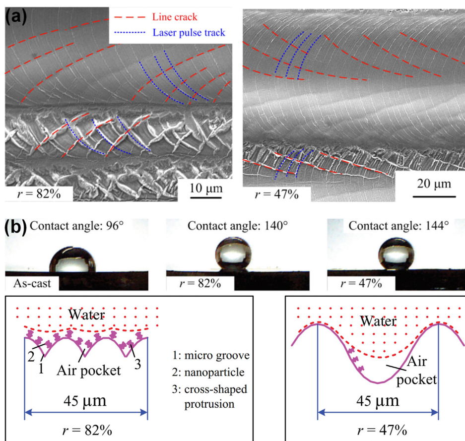
Fig. 18. (a) Surface morphology of the Zr-based BMG generated by laser processing with various pulse overlap rates r . (b) Corresponding wettability and contact status of hierarchical surfaces (Reproduced from ref. [244]).
