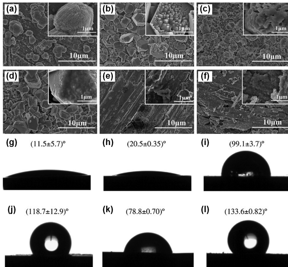
Fig. 20. Surface topography of the Ca-based BMG after different surface treatment: (a) 15 min water etching; (b) 30 min water etching; (c) 15 min water etching + FAS; (d) 30 min water etching + FAS; (e) Fe coating; (f) Fe + FAS coating. (g)–(l) The corresponding CA of the BMG surface after different treatments (Reproduced from ref. [266]).
