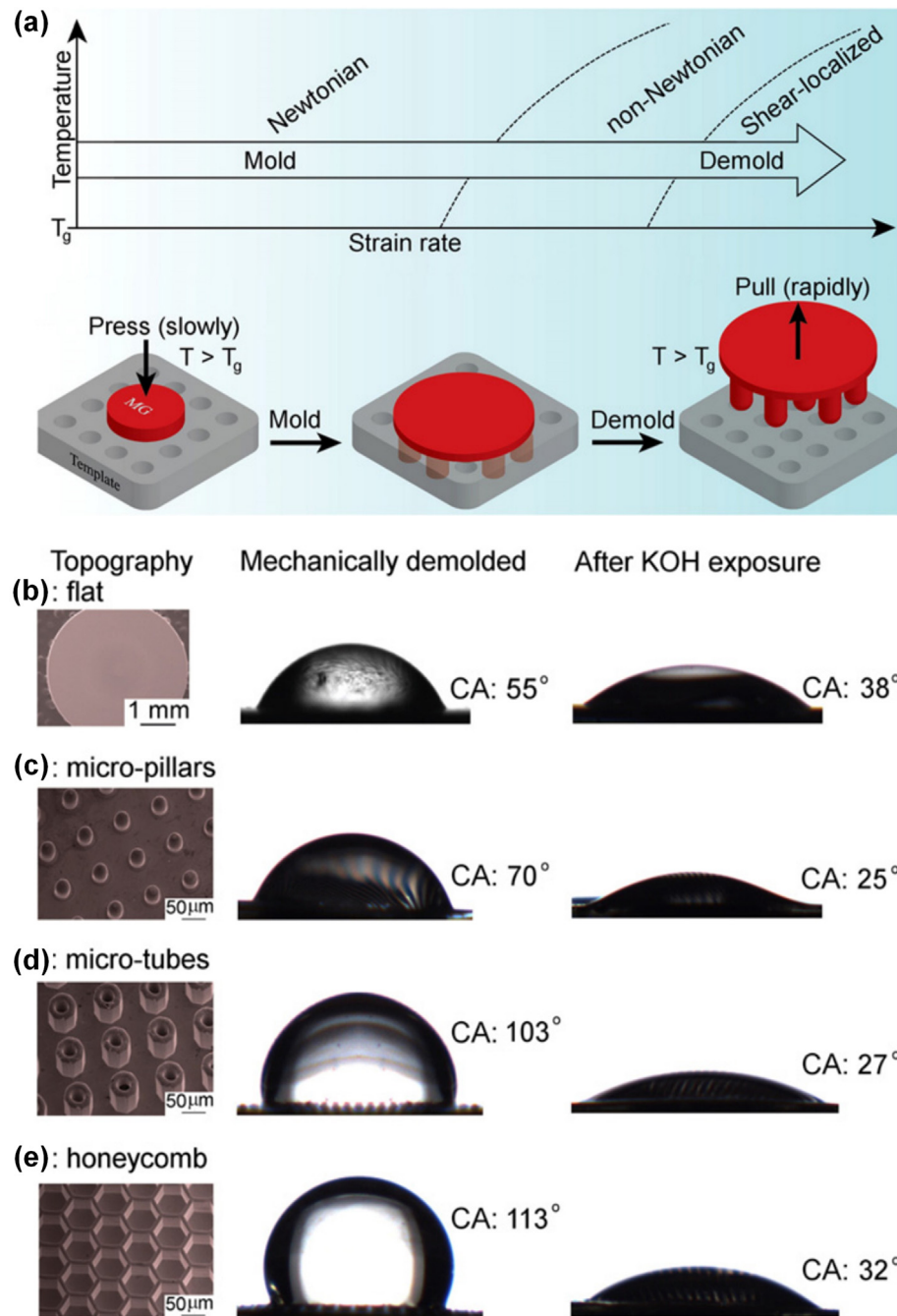
Fig. 9. (a) Forming and demolding of MG supercooled liquids at different strain rates corresponding to different flow regimes. (b), (c), (d), (e) Effect of surface structures and chemistry on the wetting behavior of the Pt-based MG, the wettability of the mechanically demolded surface evolves to hydrophobicity as the change of surface topography, while the KOH exposure obscures the topographic effects and induces hydrophilic surfaces (Reproduced from ref. [192]).
