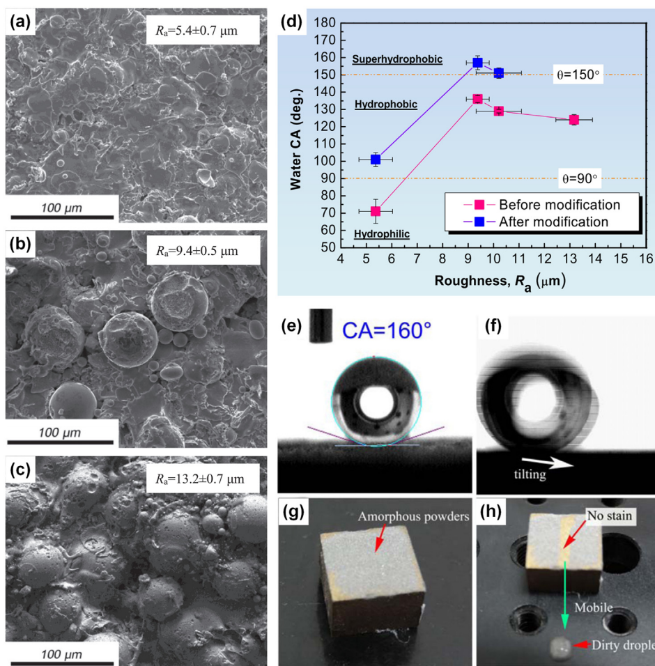
Fig. 5. (a), (b), (c) The typical morphology and surface roughness of the as-sprayed TFMGs. (d) The relation between surface roughness and water contact angle of the TFMGs with and without modification. (e), (f) The superhydrophobicity of the modified TFMGs with a contact angle of 160 degrees and a sliding angle of nearly 9 degrees. (g), (h) The self-cleaning ability of the modified TFMGs (Reproduced from ref. [132]).
