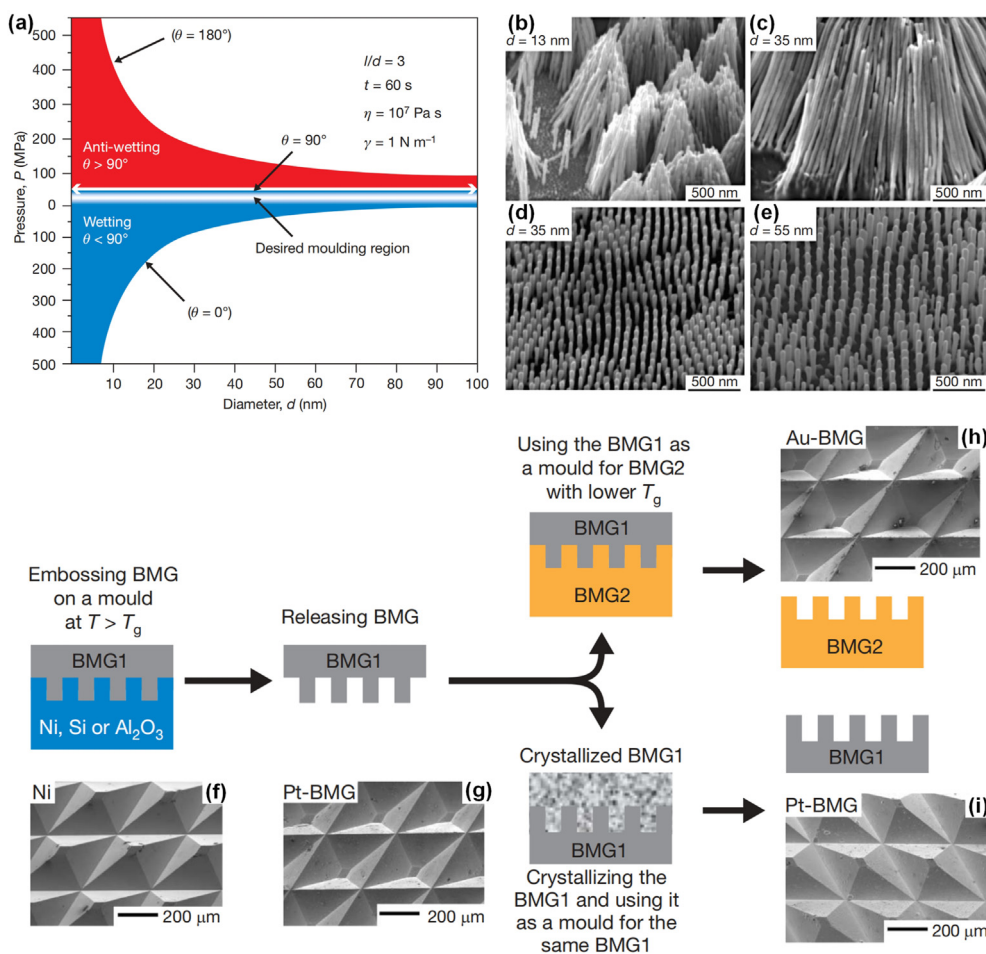
Fig. 10. (a) Forming pressure of the supercooled MGs that is required to fill the nano channels with a diameter d and an aspect ratio of 3 under both wetting ( \theta < 90^\circ ) and antiwetting ( \theta > 90^\circ ) behaviors. SEM images of nanorods formed on Pt-BMG by TPF, (b) and (c) are respectively the amorphous nanorods of diameters 13 nm and 35 nm with a high aspect ratio over 50, (d) and (e) are respectively the glassy rods of different diameters with an aspect ratio of 5. (f)–(i) The TPF process utilizing the patterned Pt-BMG as mold to fabricated surface textures on various BMGs (Reproduced from ref. [45]).
