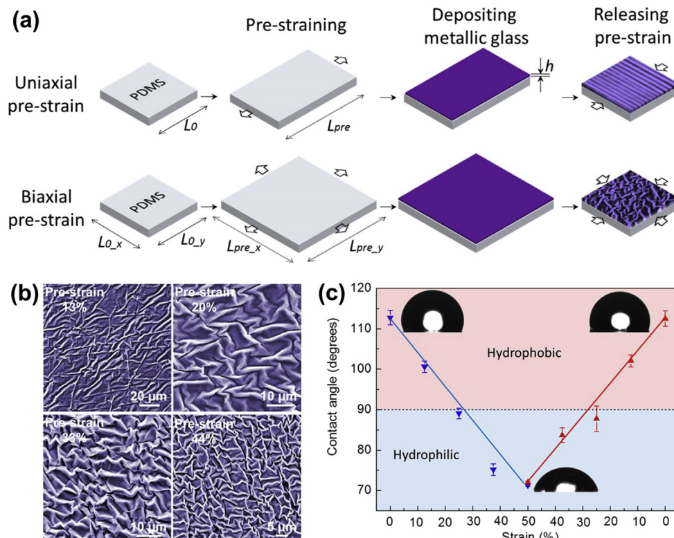
Fig. 3. (a) The folding approach for TFMGs structures fabrication. (b) Variation of the formed structures with different strains beforehand. (c) Water contact angle changes with biaxial stretching strain for the wrinkled films with initial thickness of 4 nm (Reproduced from ref. [97]).
