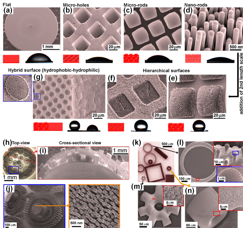
Fig. 16. Influence of the surface patterning on wetting behavior of Pt-BMG. (a) The flat sample is hydrophilic, CA = 58 degrees. (b)–(d) The patterned surfaces with single scale features remain the hydrophilicity. (g)–(e) Addition of a secondary nanostructure turn the surface to be hydrophobic with CA above 130 degrees. (h)–(j). Non-planar surface decorated with hierarchical structures fabricated by TPF and subsequent thermal blow molding. (k)–(n) 3D objects decorated with hierarchically patterned surface (Reproduced from ref. [203]).
