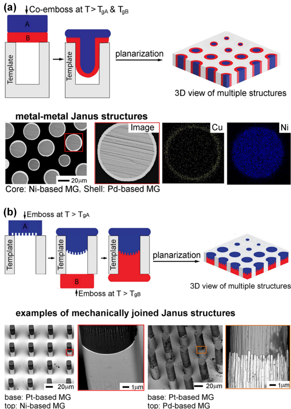
Fig. 11. (a) Fabrication of the core-shell Janus structures and interfaces through co-embossing of Ni- and Pd-based MGs. (b) Fabrication of the Janus rod arrays by thermal mechanical bonding and forming of two sets of MGs (Reproduced from ref. [197]).
