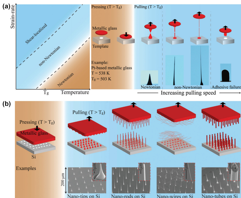
Fig. 12. (a) Regulation of the elongation behaviors of supercooled MG liquid in different flow regimes by changing the pulling speed. (b) Thermoplastic drawing processes of nanowires with various aspect ratios on BMGs (Reproduced from ref. [198]).
