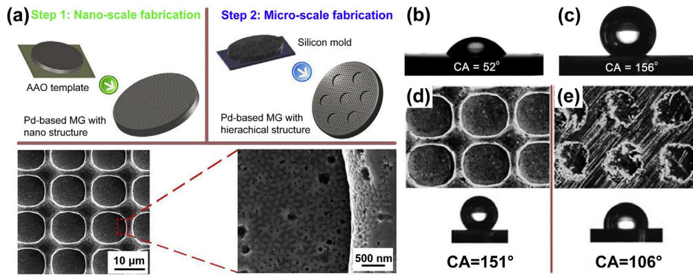
Fig. 15. (a) Formation of hierarchical features on Pd-BMG surface by the multistep TPF. (b), (c) The CA of the polished BMG surface and hierarchical BMG surface, respectively. (d), (e) The surface morphology and corresponding CA before and after sandpaper abrasion of the hierarchical structures (Reproduced from ref. [202]).
