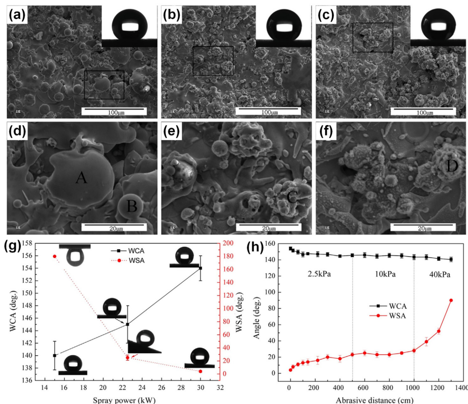
Fig. 6. Surface morphology of TFMGs (a, d), (b, e), and (c, f) at spraying power of 15, 22.5, and 30 kW respectively. (g) The wettability changes of TFMGs along with the spraying power. (h) The abrasion tests of the hydrophobic surface of TFMGs (Reproduced from ref. [134]).
