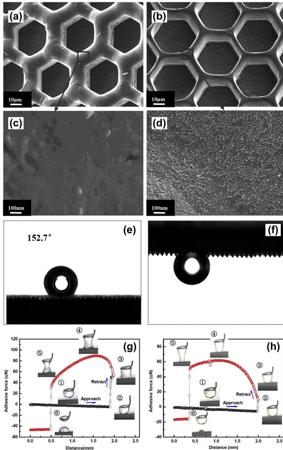
Fig. 13. SEM images of the Zr-MG surfaces with microhoneycomb structures, (a) before and (b) after etching, (c) and (d) are the corresponding images of magnified regions. (e) The CA of the hierarchically patterned MG surface. (f) The geometrical shape of water droplet on the fabricated surface at a tilt angle of 180°. (g), (h) The adhesion force of the micro/nano hierarchical surface and the surface with only microstructures, respectively (Reproduced from ref. [200]).
