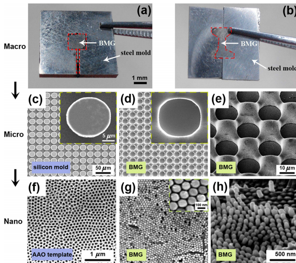
Fig. 17. Surface structures from nano- to macroscale on the Zr-based BMG fabricated by the ultrasonic assisted forming. (a), (b) BMGs fill into the rectangular hole and the dog-bone shaped hole. (c), (d), (e) scanning electron microscopy (SEM) images of the silicon molds and the microhole arrays patterned on the BMG surface. (f), (g), (h) SEM images of anode aluminum oxide (AAO) template and the formed surface with nanowires (Reproduced from ref. [218]).
