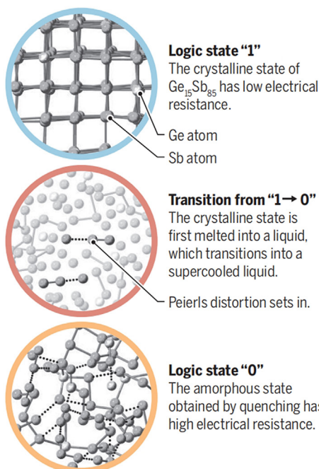
Fig. 28. The principle of PCRAM because of the amorphous phase transformation of memory arrays (Reproduced from ref. [400]).
