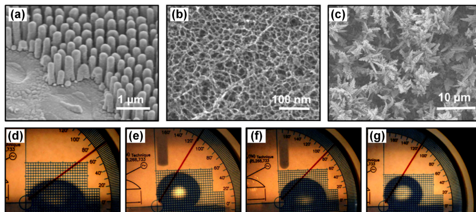
Fig. 21. Pd-based BMG surface: (a) the nanorod structure patterned by TPF, (b) the nanoporous morphology after low potential dealloying, (c) the nanodendrites formed by high potential dealloying. Water contact angle on different surfaces: (d) a flat BMG surface, (e) a nanorod patterned surface, (f) a nanoporous surface and (g) a nanodendritic surface (Reproduced from ref. [279]).
