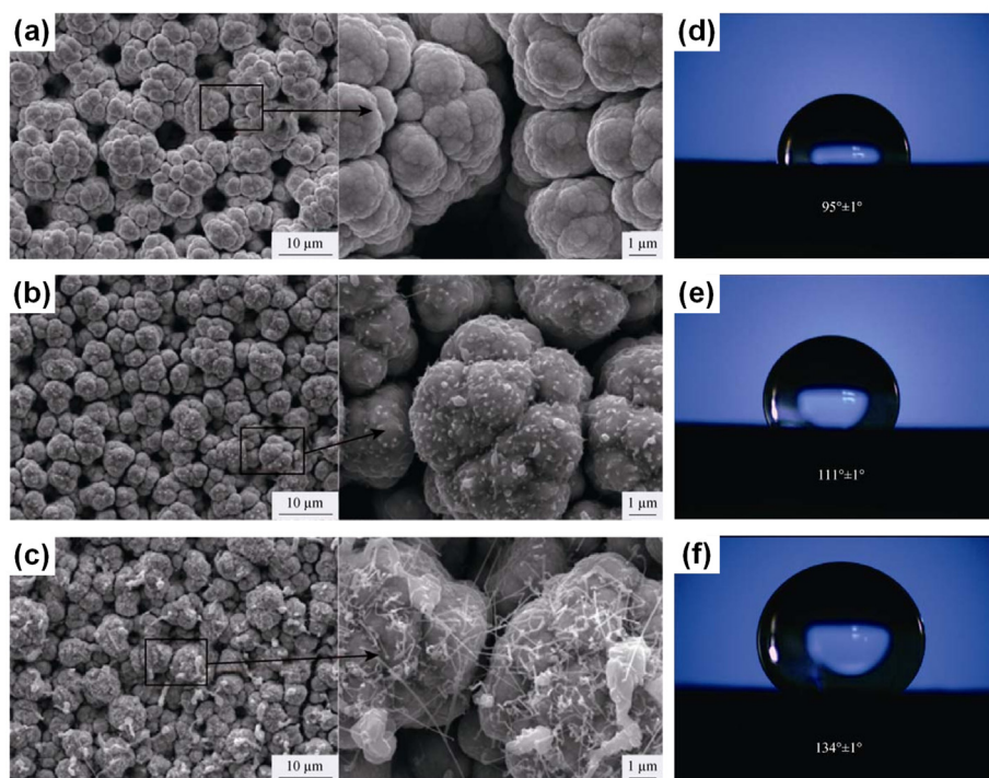
Fig. 7. Surface morphology of the TFMGs, (a) as-deposited surface, (b), (c) hierarchical surface annealed at 500 °C and 600 °C respectively. (d), (e), (f) The CA of the corresponding TFMGs (Reproduced from ref. [149]).
