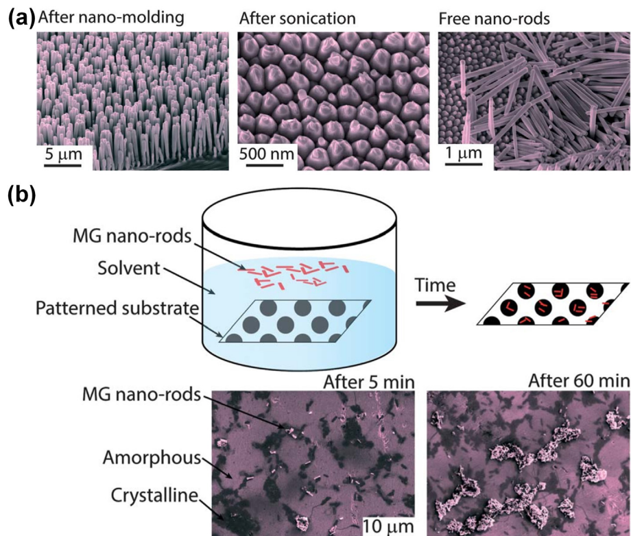
Fig. 23. (a) Fabrication of free nanorods by the sonication processing of patterned MGs. (b) Self-assembly of the free nanorods of MGs that may be driven by the effect of crystal-field, and the nanorods tend to gather in the crystalline regions (dark) rather than the amorphous region (light) (Reproduced from ref. [48]).
