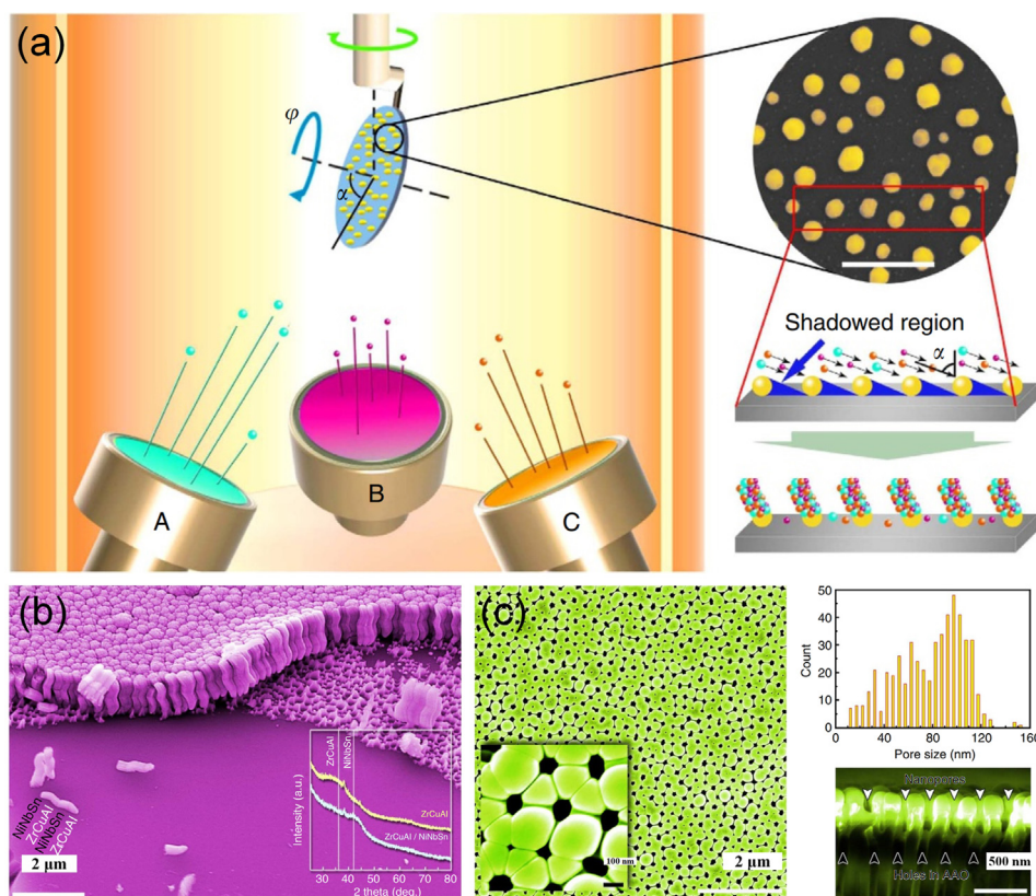
Fig. 4. (a) Multitarget carousel oblique angle deposition. (b) Hybrid nanostructures comprising two kinds of metallic glasses. (c) Nanoporous metallic glass membrane (Reproduced from ref. [103]).
