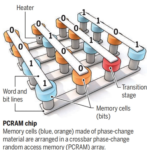
Fig. 28. The principle of PCRAM because of the amorphous phase transformation of memory arrays (Reproduced from ref. [400]).
