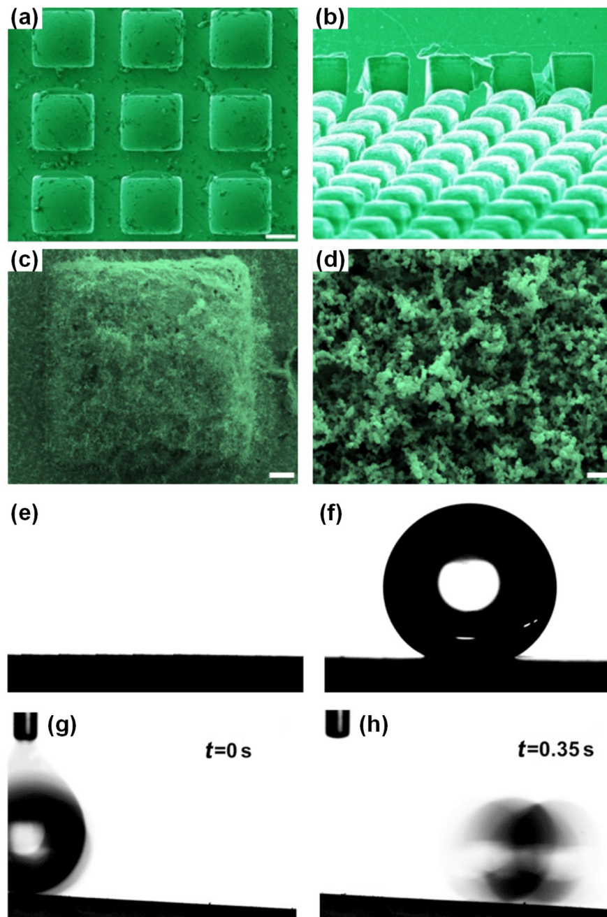
Fig. 14. (a) The top view of a regular array of square micropillars formed on the Ce-based BMGs. (b) The cross-sectional image of the patterned surface. (c), (d) ESEM images of the hierarchical surface structures after the SiO 2 /soot deposit at different magnification. (e), (f) The CA of the as-patterned BMG surface and the hierarchical surface after deposition, respectively. (g), (h) The contact process of a water droplet on the hierarchical surface of BMGs with a small sliding angle (Reproduced from ref. [201]).
