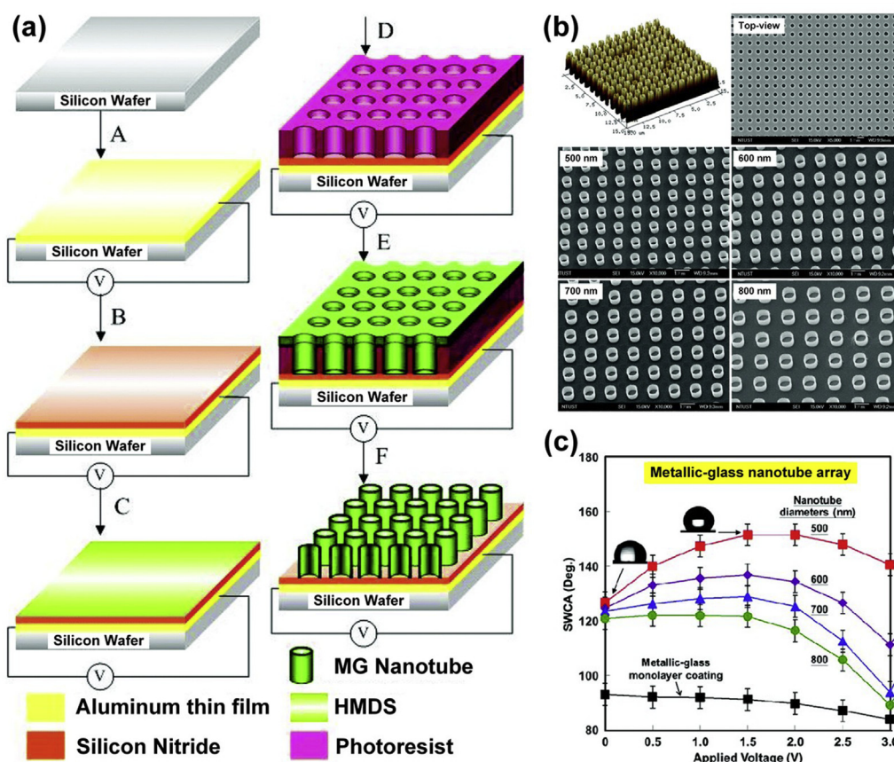
Fig. 1. (a) The fabrication process of the TFMG nanotube arrays. (b) AFM and SEM image nanotube arrays with different diameters. (c) Variation of the CA of the nanotube arrays and the plate TFMGs along with the heating voltages (Reproduced from ref. [93]).
