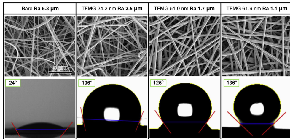
Fig. 2. Water contact angle of bare and coated membrane with various coating thickness of TFMGs (Reproduced from ref. [95]).
