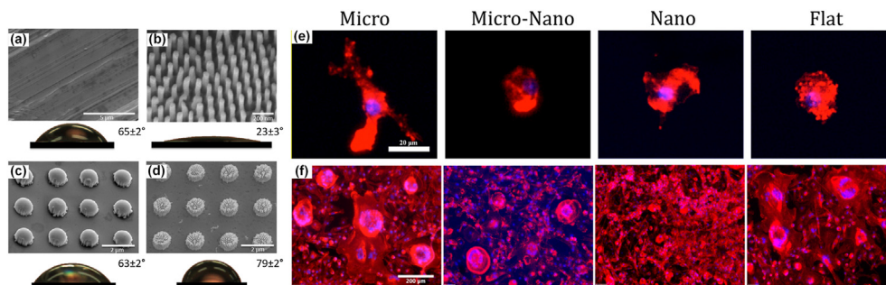
Fig. 26. Influence of surface patterns on the water contact angles for Pt-BMG, (a) flat surface, (b) nanopatterned surface, (c) micropatterned surface, (d) micro-/nanohierarchical surface. The cell responses and immunofluorescence images of macrophage fused on different MG surfaces, (e) low magnification images, (f) high magnification images (Reproduced from ref. [383]).
