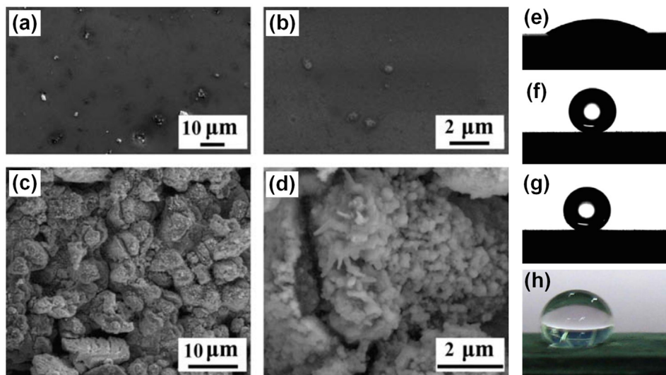
Fig. 19. (a), (b) The original surface of CaLi-based BMG surface. (c), (d) Hierarchical surface generated by the treatment of etching and FAS coating. (e) Water droplet on the original surface. (f) Water droplet on the etched and modified surface with a CA of 162 degrees. (g) Oil droplet on the treated surface with a CA of 156 degrees. (h) A water droplet on the treated BMG surface after exposure to air for three months (Reproduced from ref. [264]).
