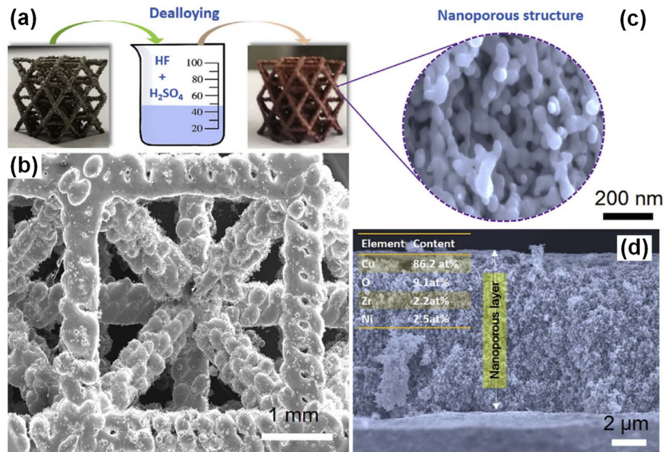
Fig. 22. (a) The Zr-based MG lattice fabricated by 3D printing before and after chemical dealloying for 60 h in the acid solution. (b) SEM morphology of the as-prepared lattice structures. (c) Fabrication of the nanoporous structures on the as-prepared MG lattice by dealloying. (d) Cross-section morphology of the uniform nanoporous layer around 10 μm-thick (Reproduced from ref. [287]).
