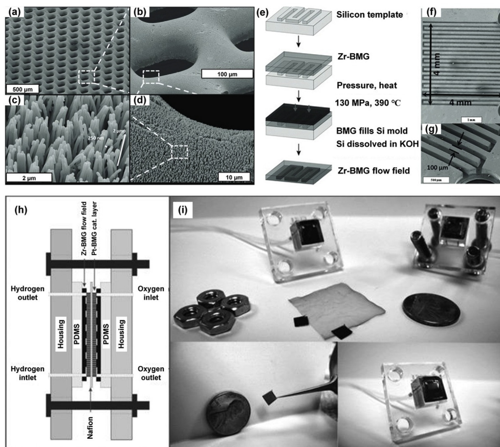
Fig. 27. (a)–(d) The nanowire electrode of Pt-BMG with gas feeding holes formed by multistage TFP. (e)–(g) Zr-BMG flow fields formed by TFP. (h) (i) Microfuel cell using the catalytic layers of porous Pt-BMG nanowires, and the flow field/current collector plates of Zr-BMG (Reproduced from ref. [55]).
