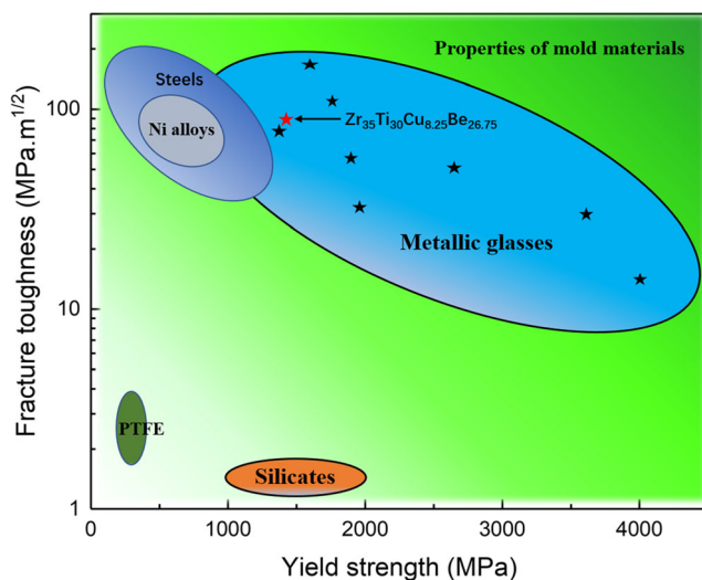
Fig. 5 The yield strength versus fracture toughness of some commonly used materials for injection mold inset. Including Silicates, PTFE, Ni alloys, Steels and metallic glasses, among them, the Red Pentagram pattern is the material of this experiment
