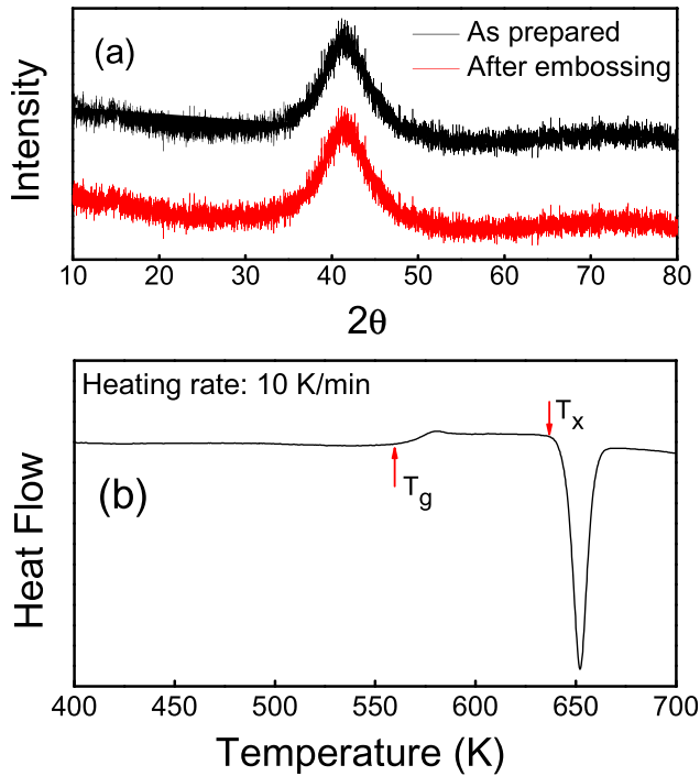
FIG. 1. (a) XRD patterns of the as prepared and embossed \text{Pd}_{40}\text{Cu}_{30}\text{P}_{20}\text{Ni}_{10} metallic glass. (b) DSC scans (at a heating rate of 10 K/min) of the Pd-based BMG.
