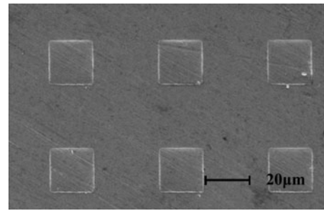
FIG. 5. SEM image of square array on the surface of Sr-based BMG imprinted at room temperature.
