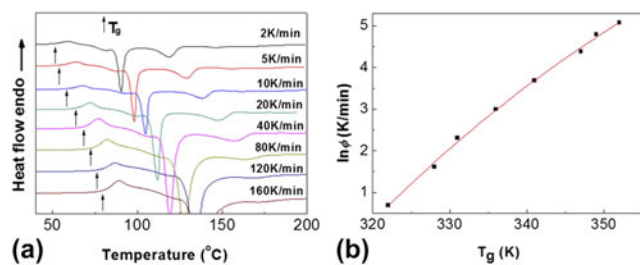
FIG. 3. (a) DSC curves of \text{Sr}_{60}\text{Mg}_{18}\text{Zn}_{22} BMG at different heating rate and (b) VFT relation between glass transition temperature T_g and heating rate \phi of \text{Sr}_{60}\text{Mg}_{18}\text{Zn}_{22} BMG.
