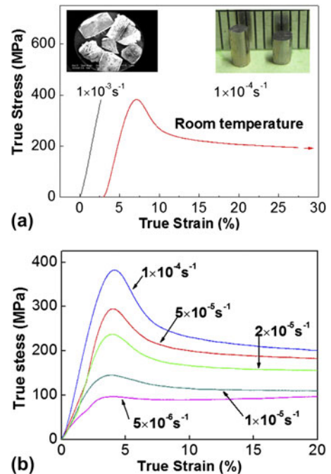
FIG. 6. (a) Different deformation type of \text{Sr}_{20}\text{Ca}_{20}\text{Yb}_{20}\text{Li}_{11}\text{Mg}_9\text{Zn}_{20} BMG at room temperature. The inset at left shows that the BMG is brittle at high strain rate, while the inset at right shows that the BMG is superplastic at low strain rate. (b) Stress–strain curves of \text{Sr}_{20}\text{Ca}_{20}\text{Yb}_{20}\text{Li}_{11}\text{Mg}_9\text{Zn}_{20} BMG at different strain rate.
