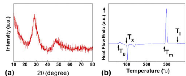
FIG. 1. (a) XRD pattern of the as-cast \text{Sr}_{60}\text{Mg}_{18}\text{Zn}_{22} BMG. (b) DSC curve of the as-cast \text{Sr}_{60}\text{Mg}_{18}\text{Zn}_{22} BMG.
